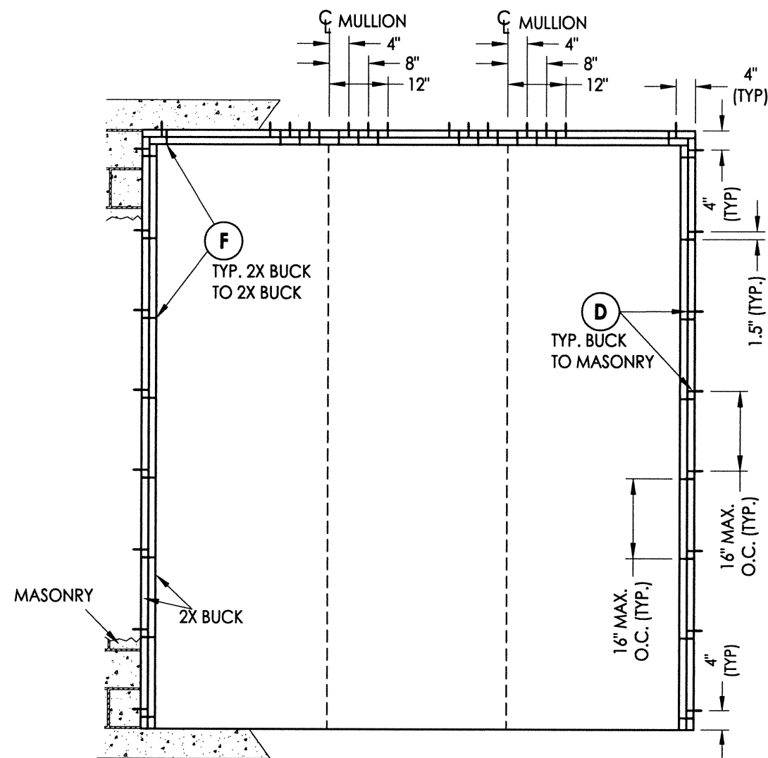
BUCK ANCHORING OXO
