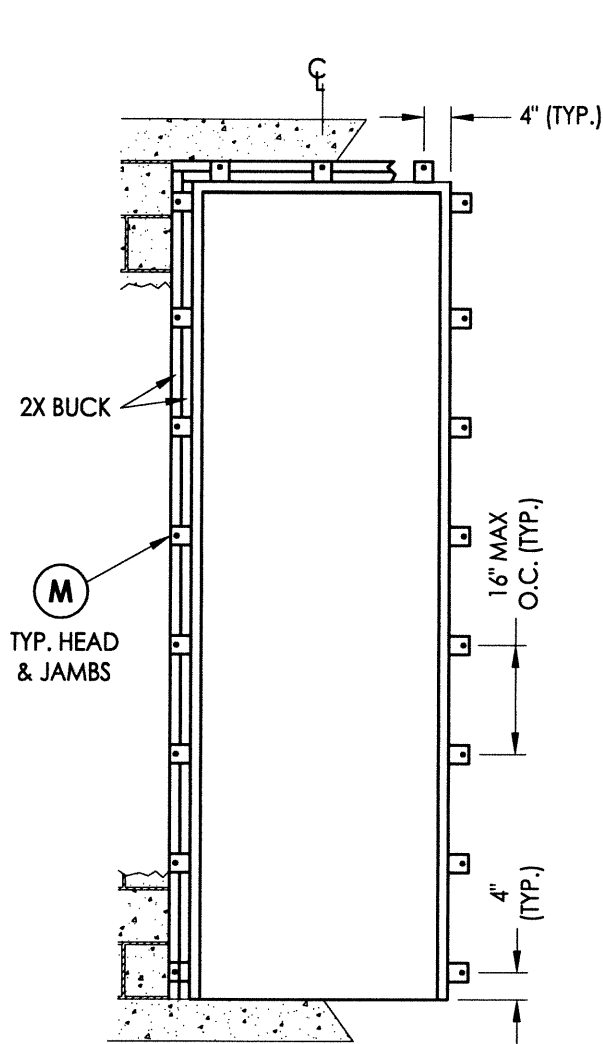
FRAME ANCHORING X
