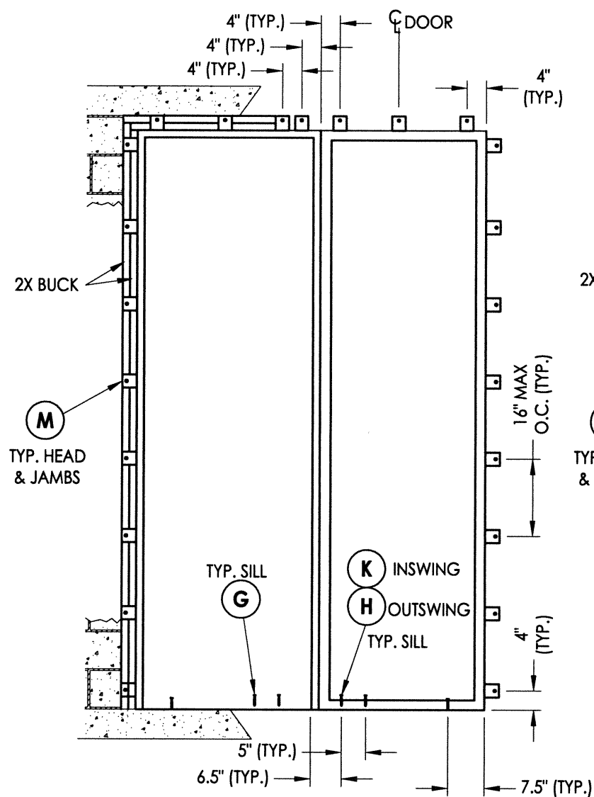
FRAME ANCHORING XX
