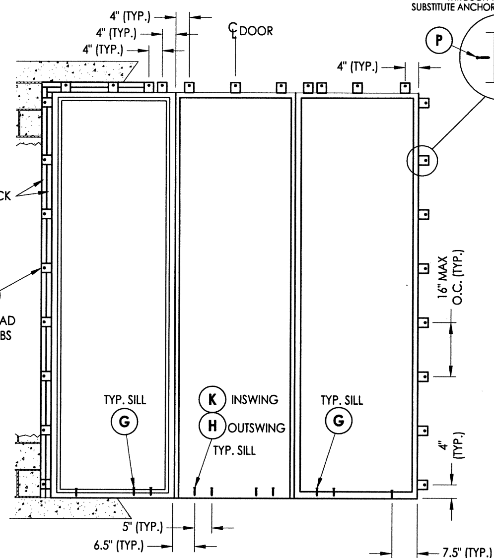
FRAME ANCHORING OXO
