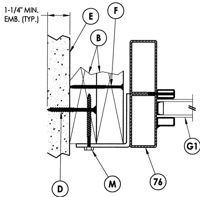
1 6 HORIZONTAL CROSS SECTION
